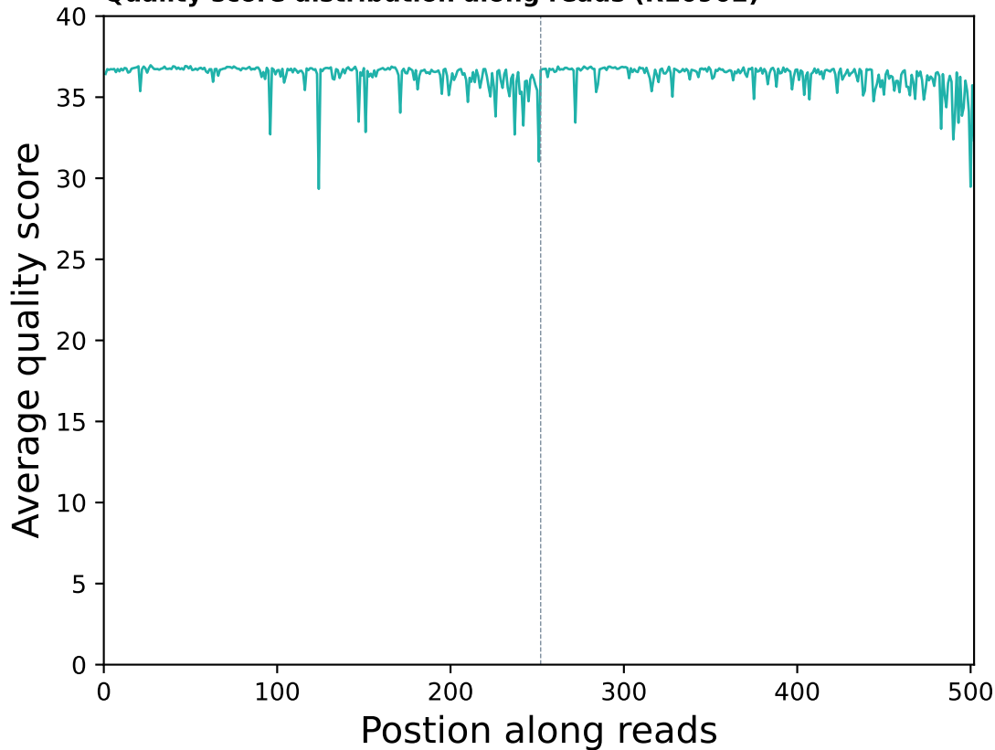
Quality score distribution along reads (R10902)
